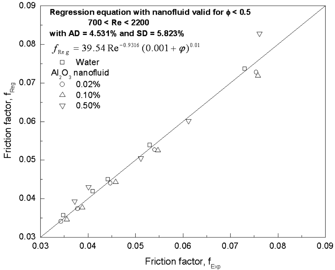
Figure 8. Comparison of experimental friction factor with Eq. (9).
